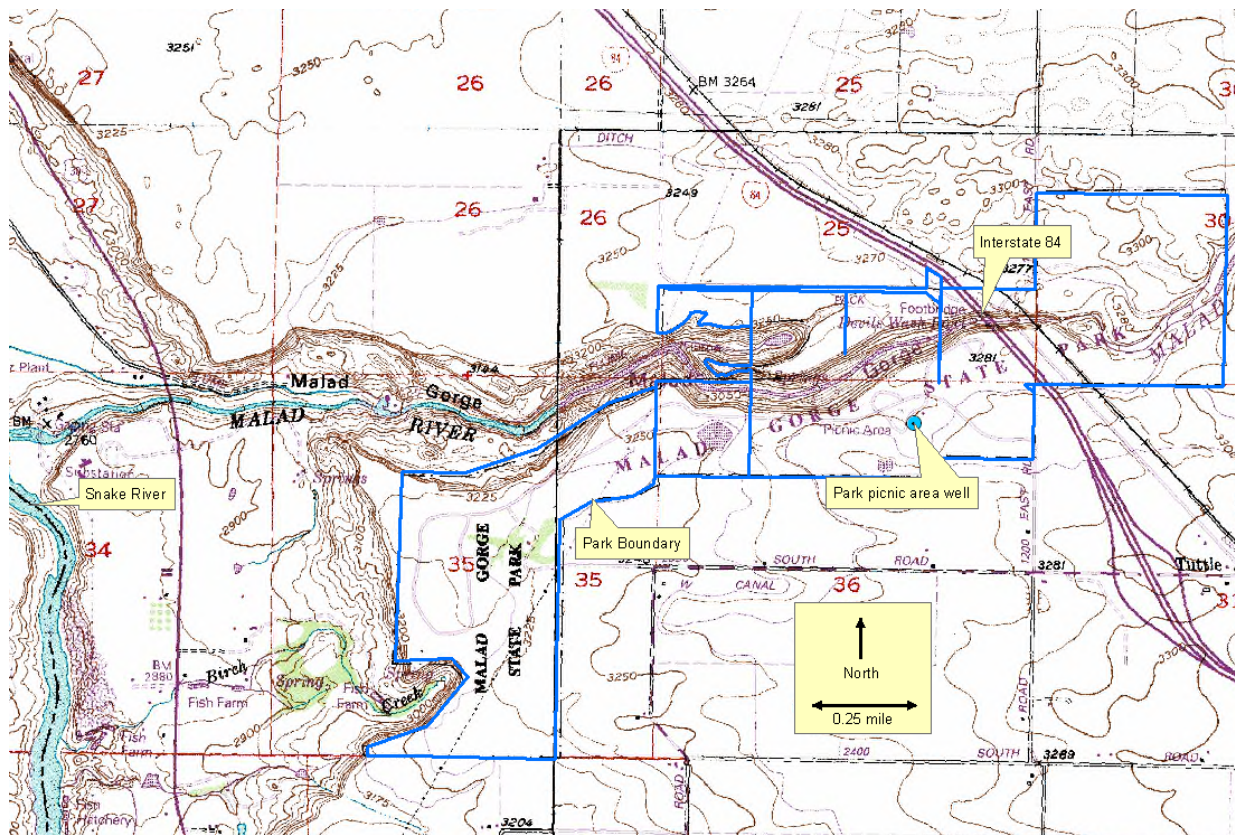
Figure 2. USGS topographic map of the site showing the park boundary as the blue colored line.
