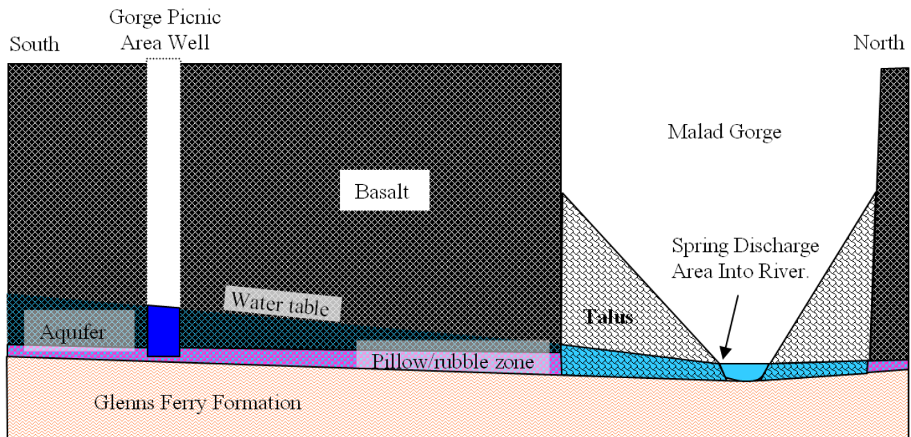
Figure 7. General conceptual cross section geologic model for the tracer test area (not to scale).
