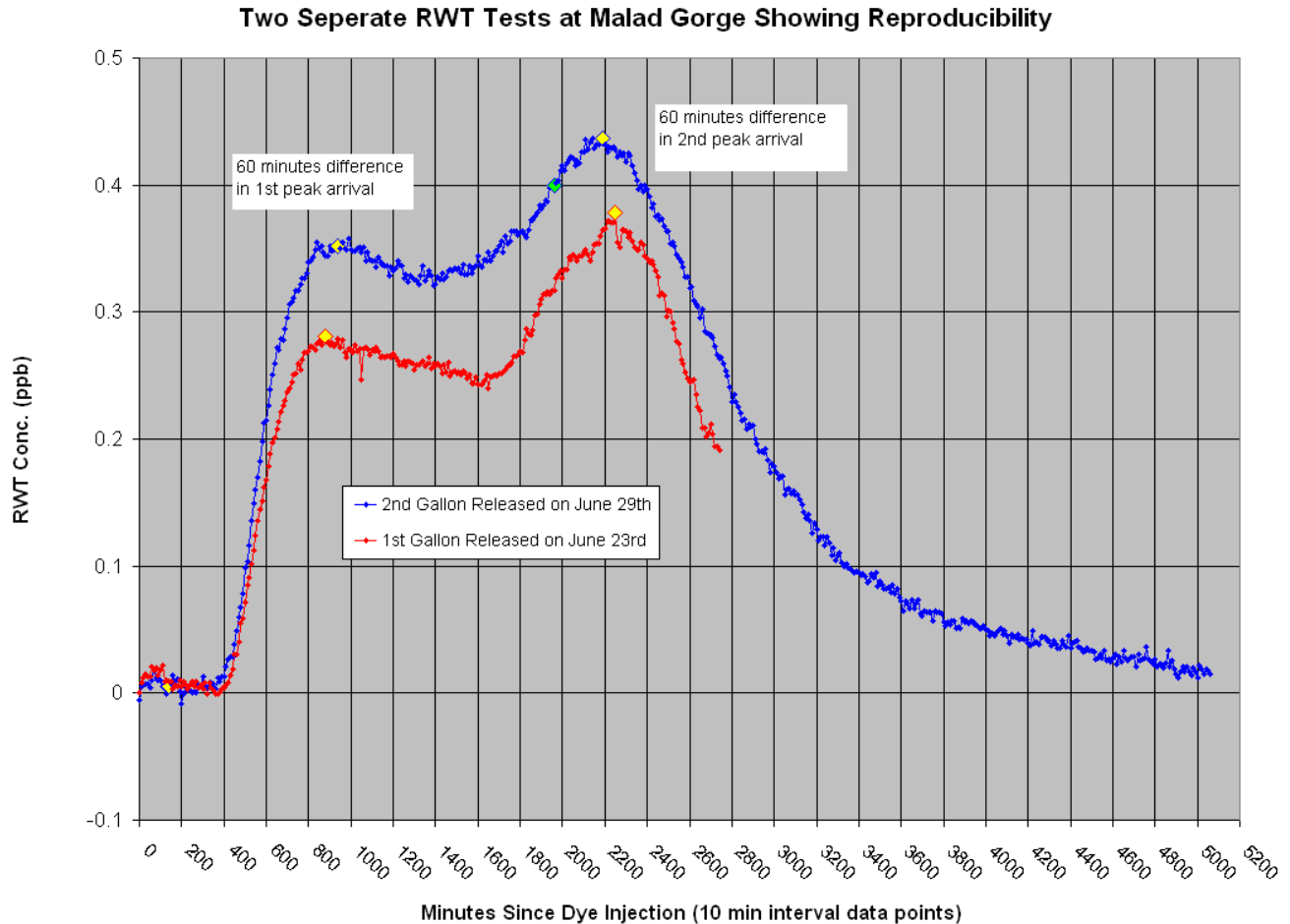
Figure 17. Reproducibility of both RWT tests demonstrating similar patterns with a strong correlation.
