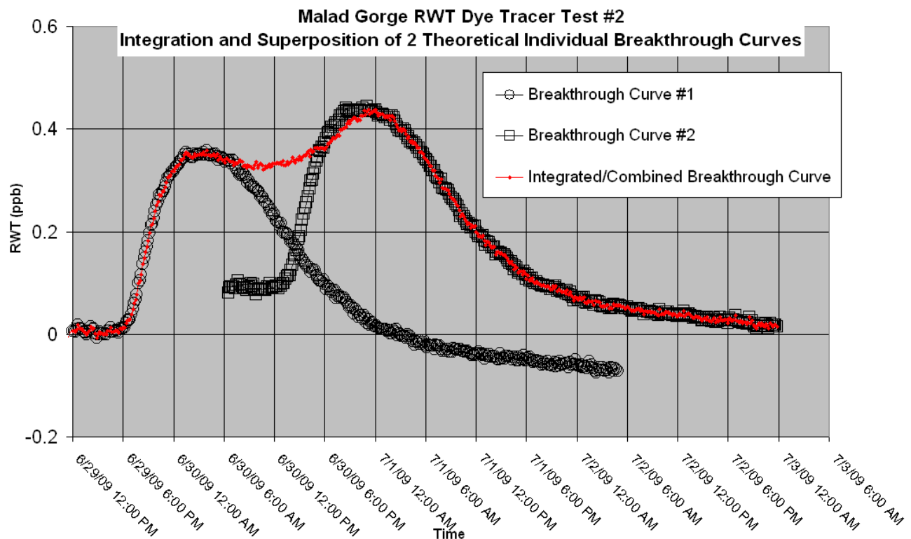
Figure 16. A general combination of two individual conceptualized concentration breakthrough curves noted in black with circles for Curve #1 and squares for Curve #2. The integration of these two black symbol curves would have the shape of the red symbol line.
