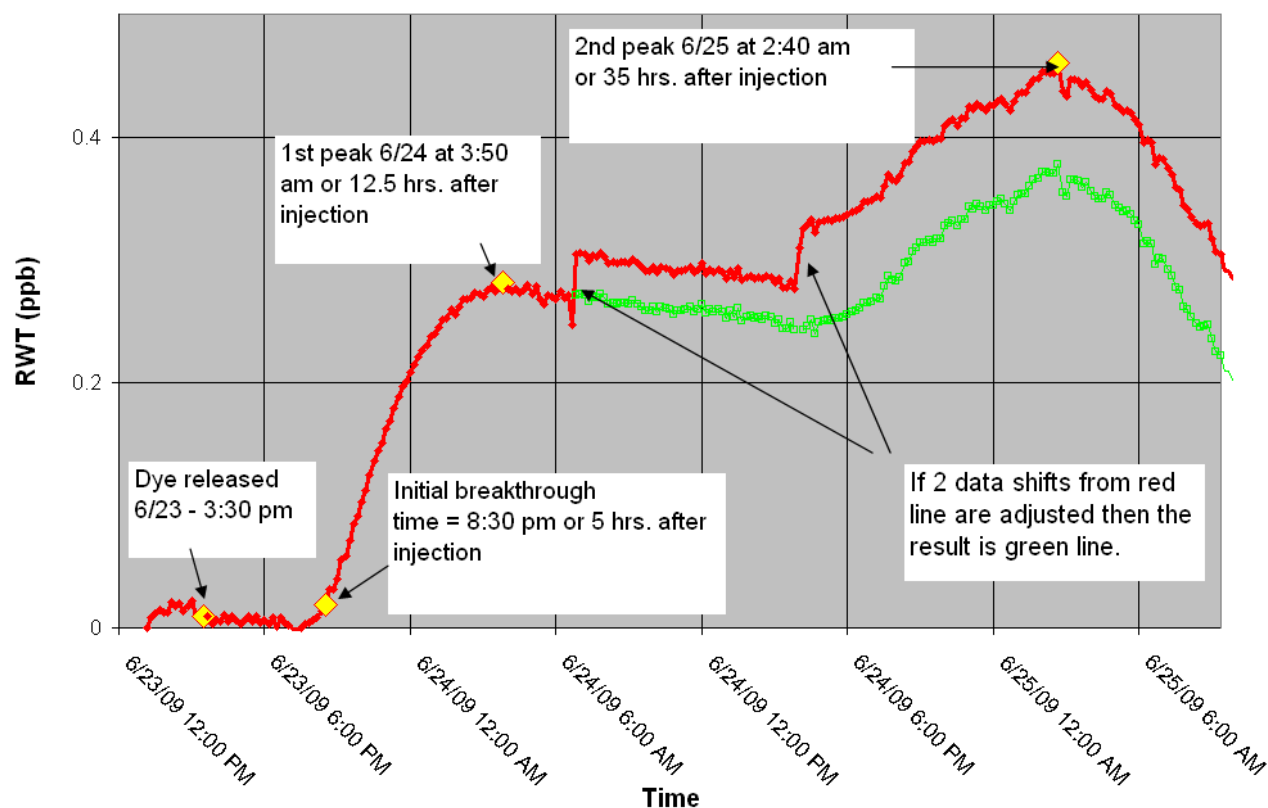
Figure 14. Expanded view of the oval shaped circled data in Figure 13 concentration breakthrough curve. Note the two peaks and temporal pattern for comparison with the second RWT test. Two data shifts occurred and if adjusted then the green line would be the resultant curve.
