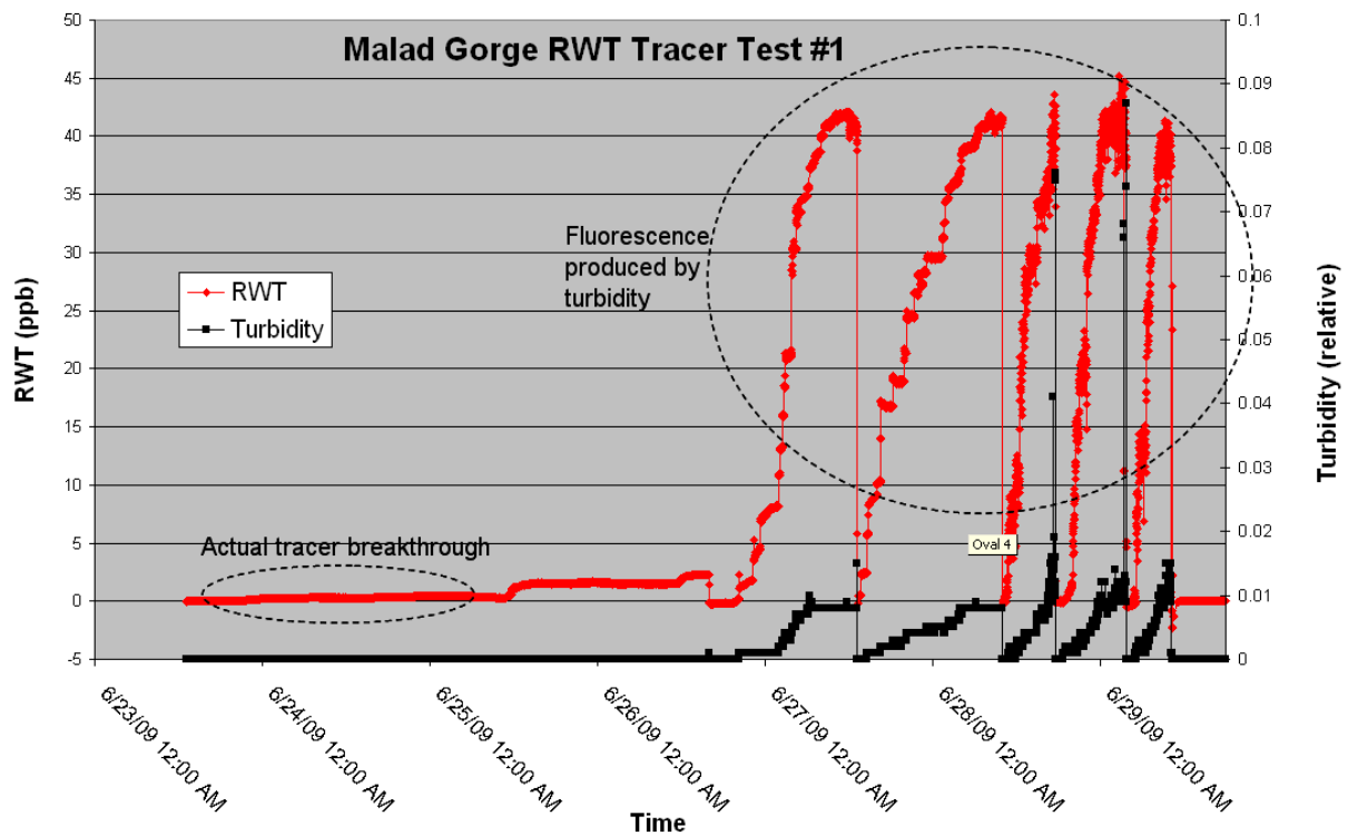
Figure 13. RWT test #1 concentration breakthrough curve from SCUFA. Fluorescent spikes correlate to turbidity spikes.
