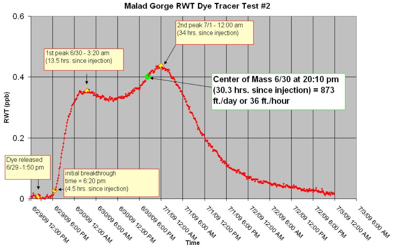
Figure 15. Dye concentration breakthrough curve for 2 nd RWT test. Note the same two peak pattern as in test #1 confirming reproducibility.
