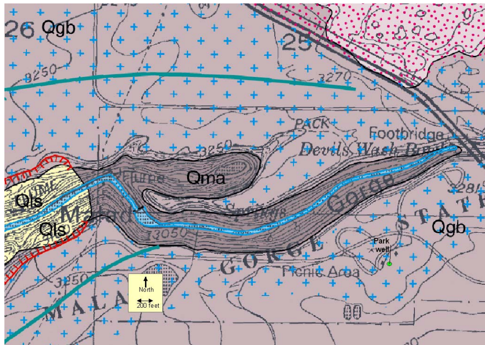
Figure 3. Geologic map showing the upper section of Malad Gorge Pleistocene age basalts Madson (Qma) and Gooding Butte (Qgb) (Gillerman et al, 2005). See Appendix A.
