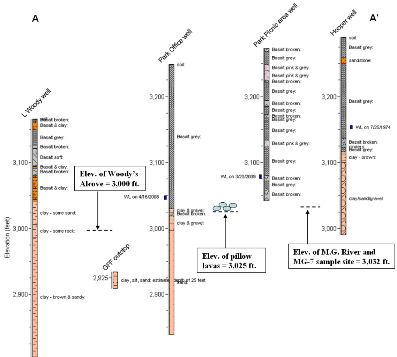
Figure 6. Geologic cross section A-A' noting sediments as orange colored background and basalt related rock type as grey colored background patterns. Elevations of Woody's Alcove, pillow basalt outcrop and the Malad Gorge River/sample site MG-7 are also shown. Tick marks are every 25 feet. Well water levels are shown with dates.
