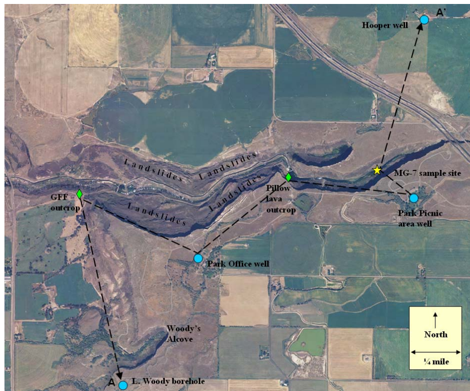
Figure 5. Location of geologic cross section line A-A' with wells noted as blue circles, outcrops as green diamonds and sample site MG-7/Malad River as yellow star.
